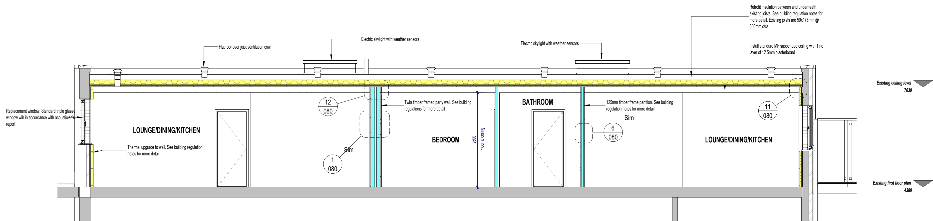
2 Section B-B 1:50
