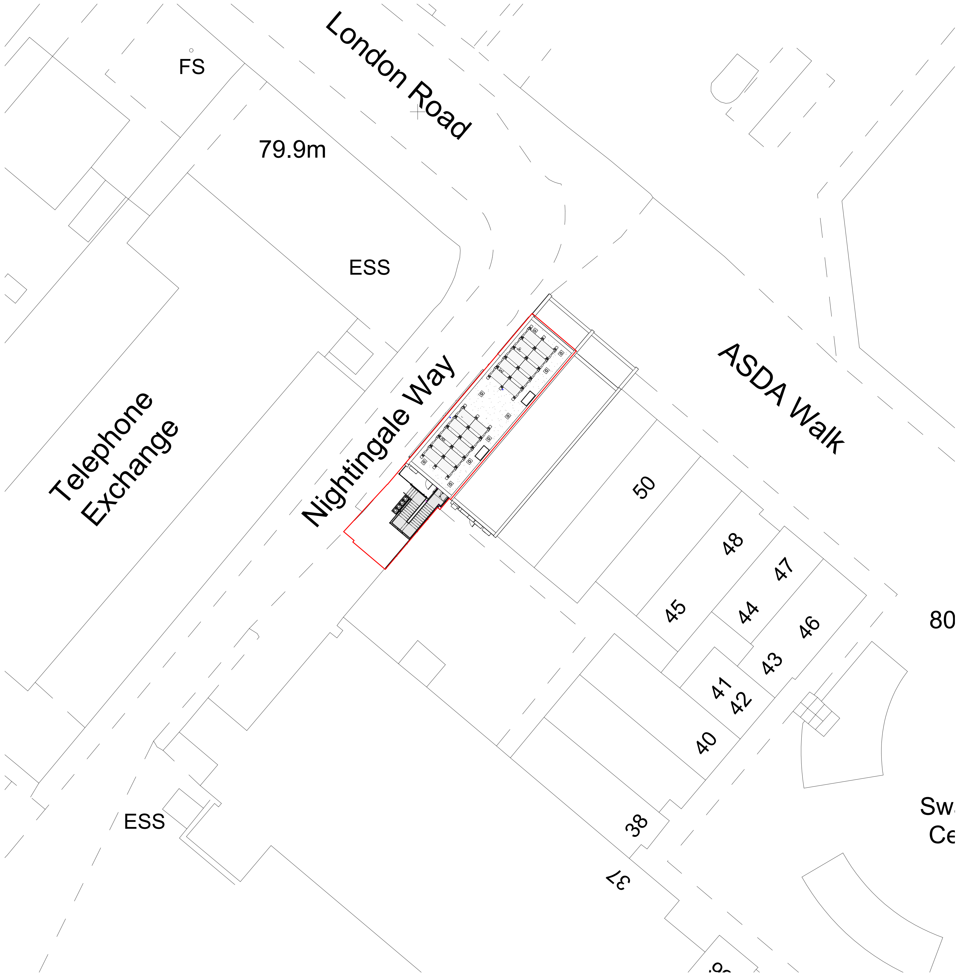
1 Proposed block plan 1 : 200
