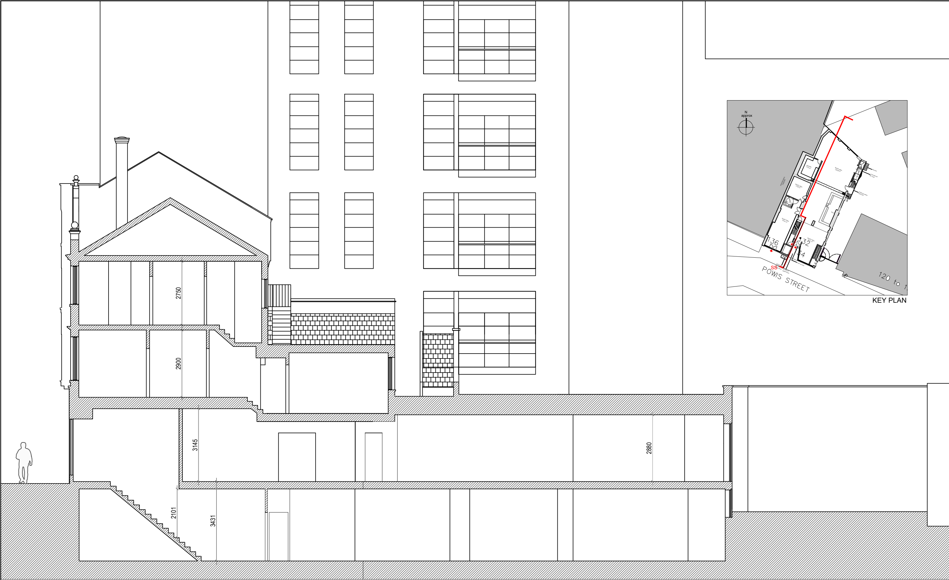
PROPOSED SECTION SCALE 1:100
