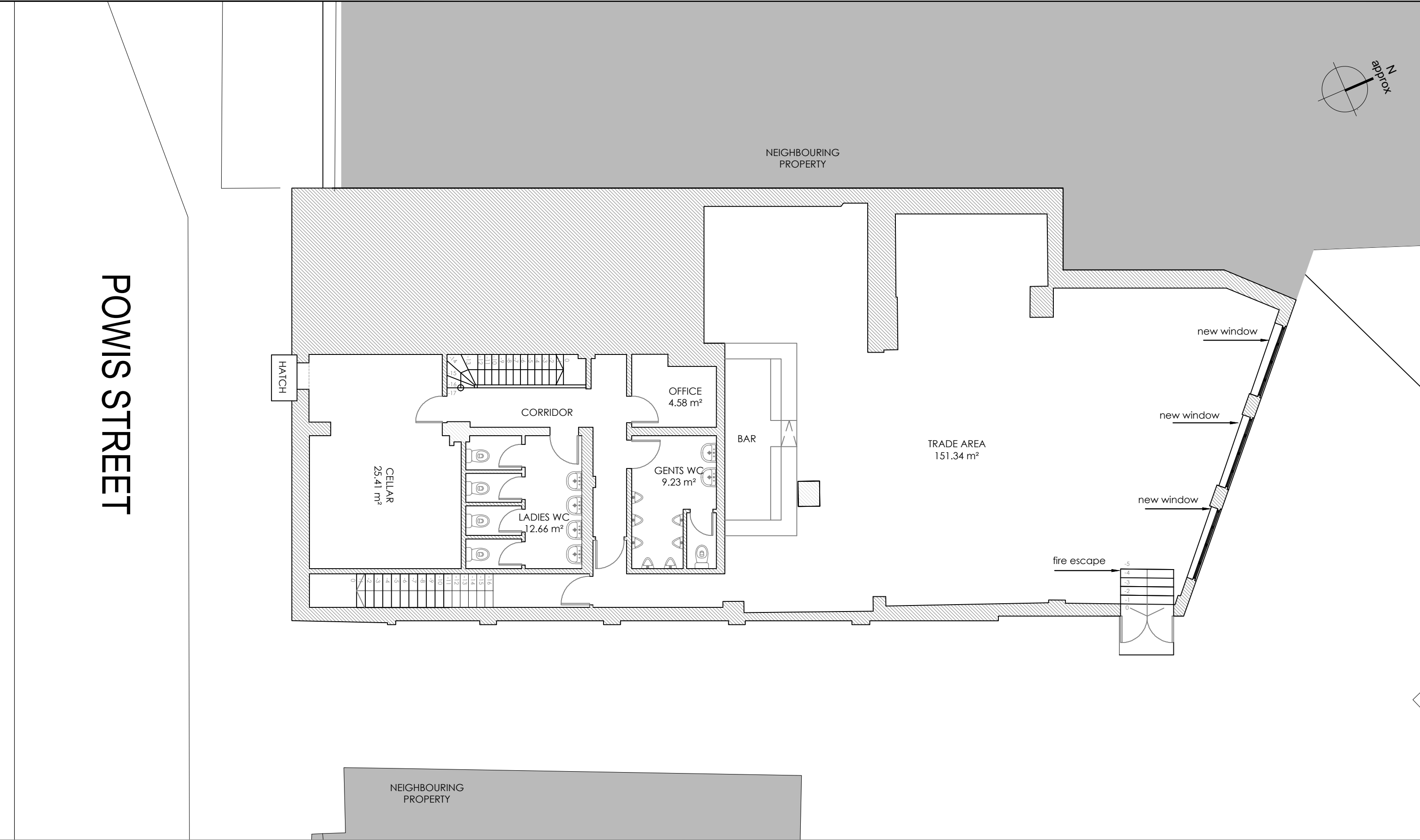
PROPOSED BASEMENT SCALE 1:100
