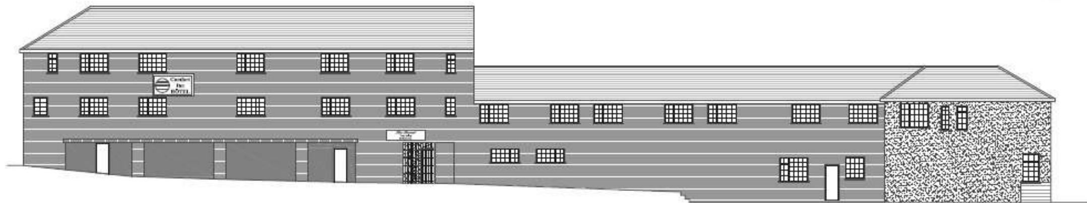
Rear Elevation As Existing
