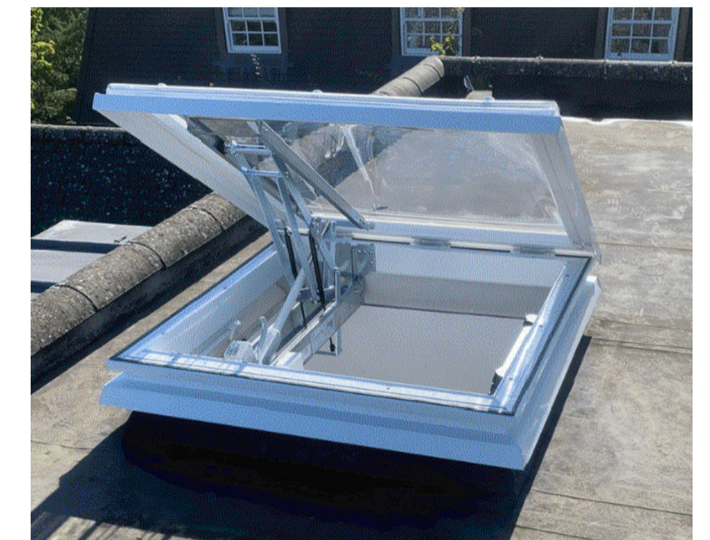
Proposed Vent Type B Proprietary Fully Operable Glazed Vent to Head of Stairs and Seventh Floor Corridors Size to Suit Opening
