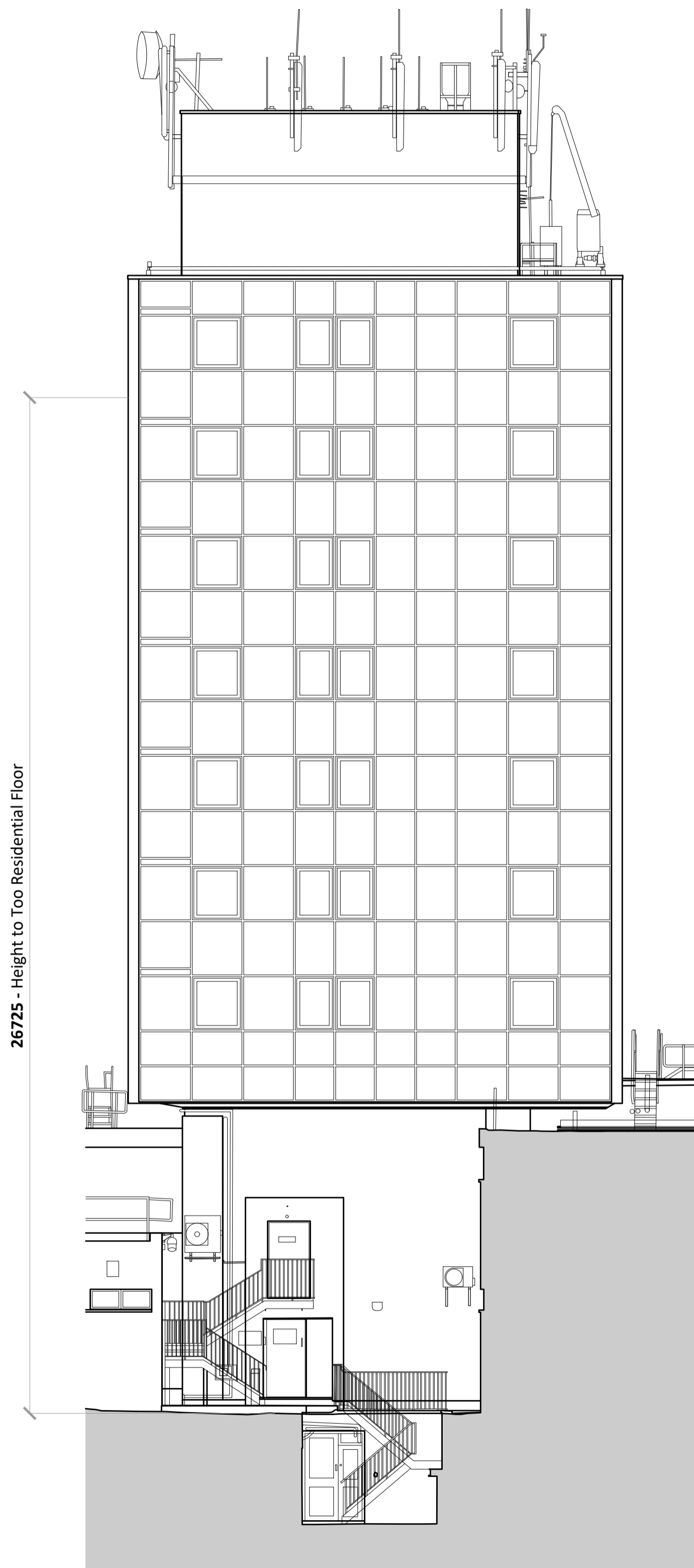
Existing & Proposed | Elevation 01
