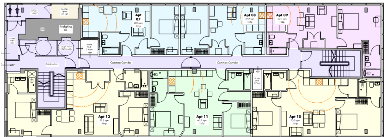
Figure 6: Proposed Second Floor Level
