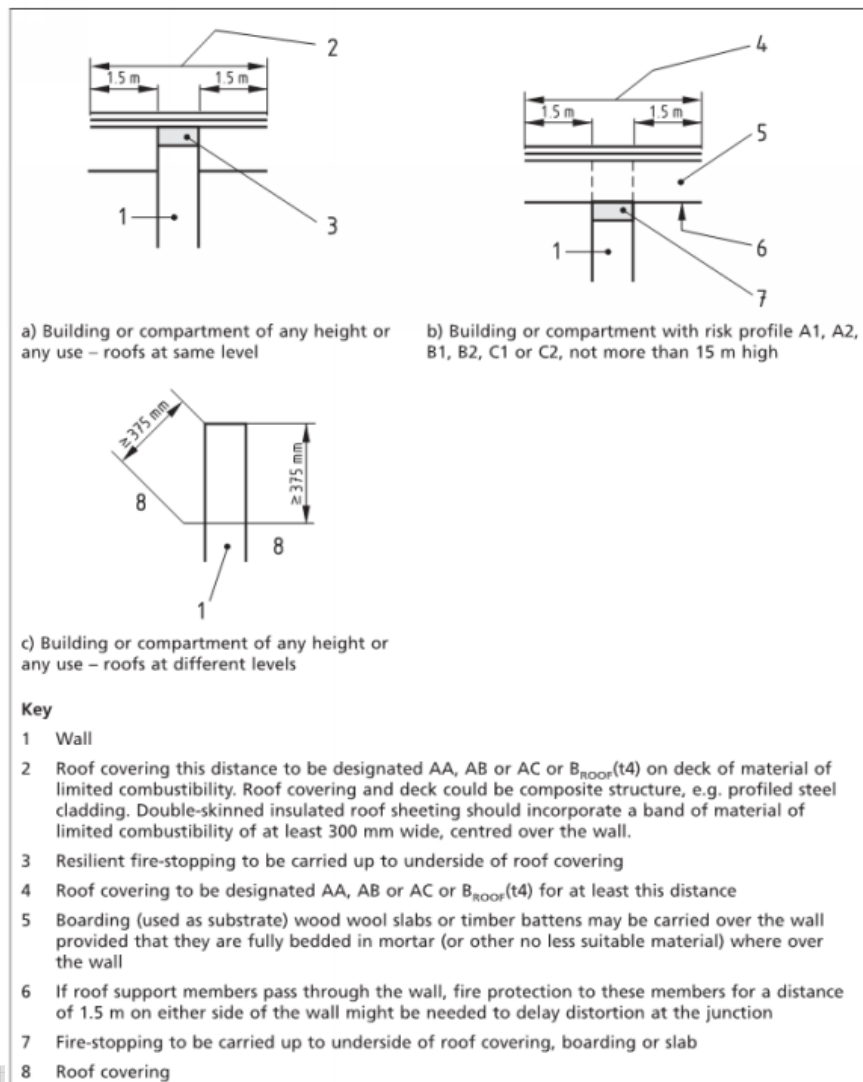
Figure 19: Junction of Compartment Wall and Roof
