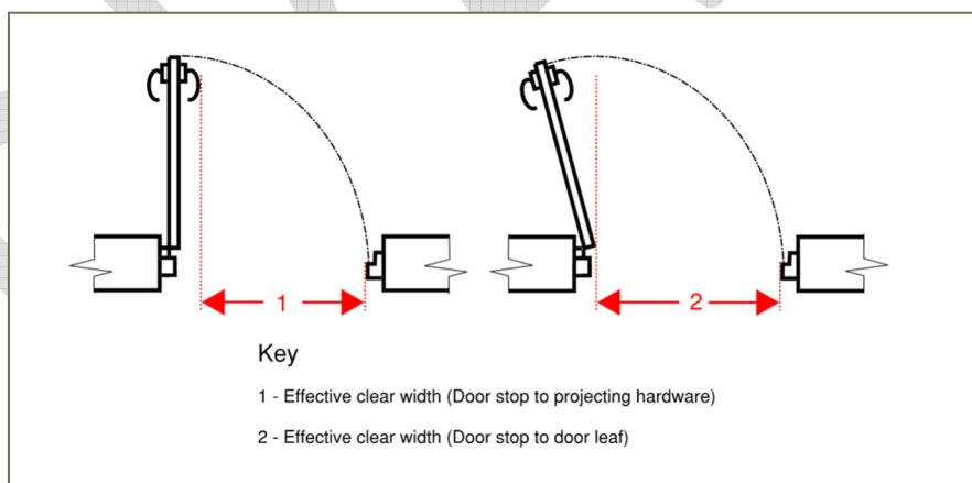
Figure 17: Clear Exit Width
