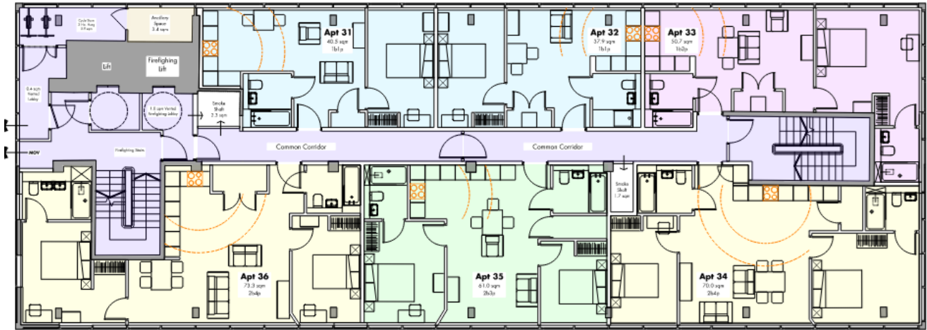
Figure 10: Proposed Sixth Floor Level
