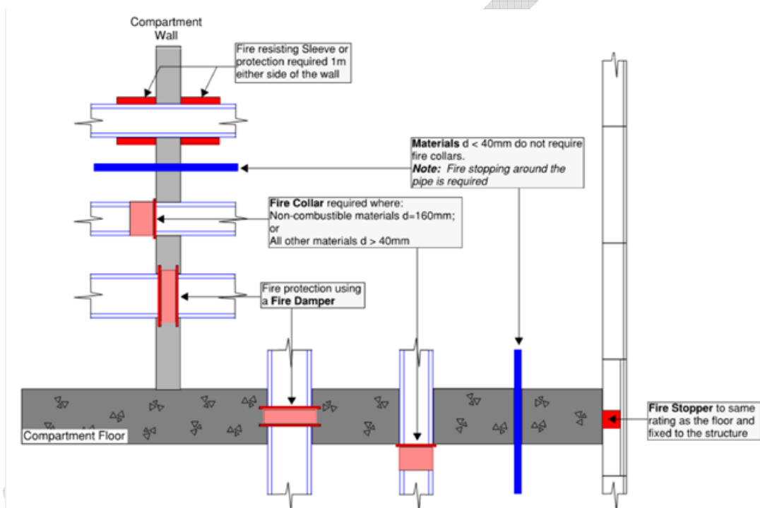
Figure 21: Protection of Openings and Fire Stopping
