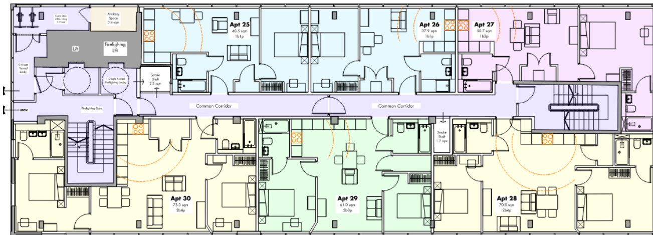
Figure 9: Proposed Fifth Floor Level
