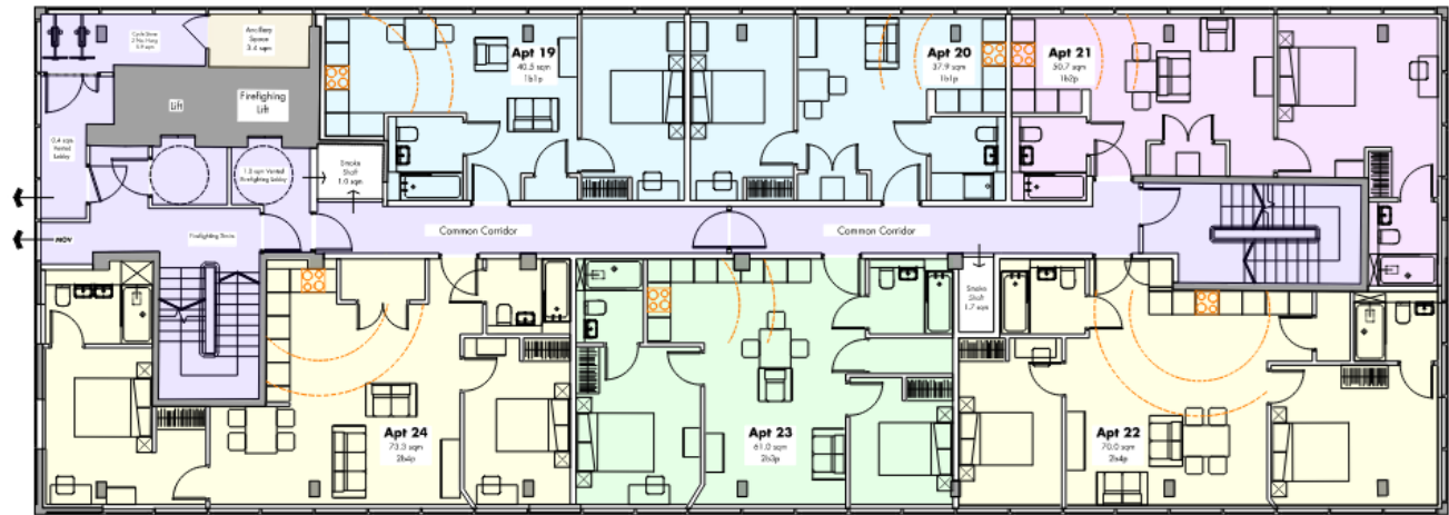
Figure 8: Proposed Fourth Floor Level
