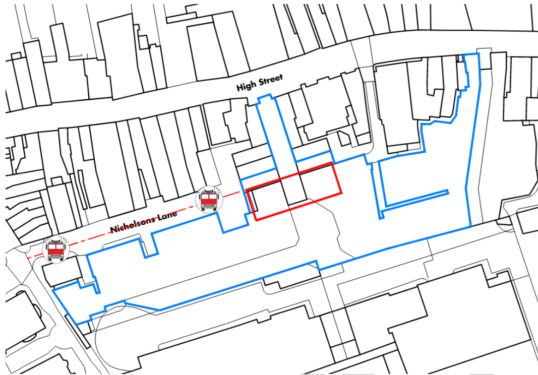
Figure 23: Fire Service Access
