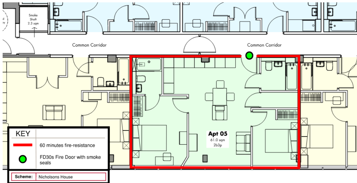
Figure 18: Compartmentation – Example of Apartment Layout
