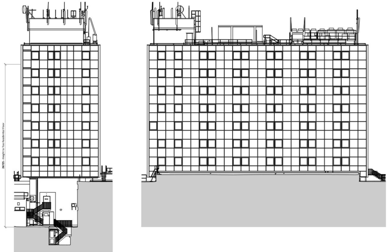
Figure 13: Proposed Elevations 1 & 2
