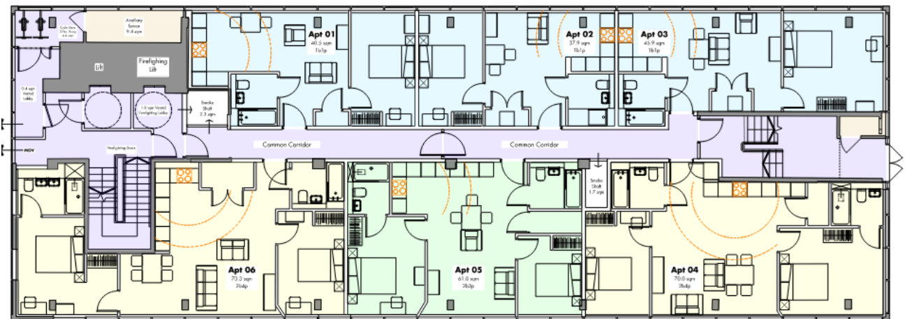
Figure 5: Proposed First Floor Level
