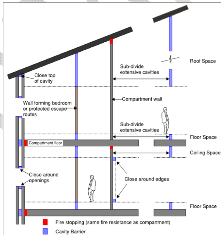
Figure 20: Junction of Compartment Wall and Roof
