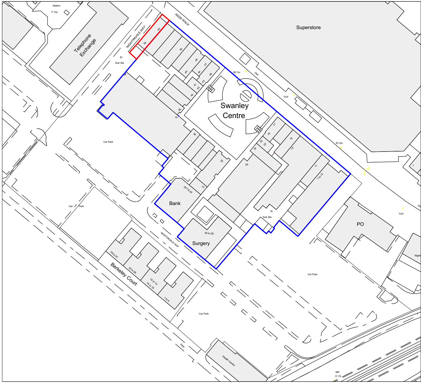
1 Site Location Plan Scale: 1:1250
