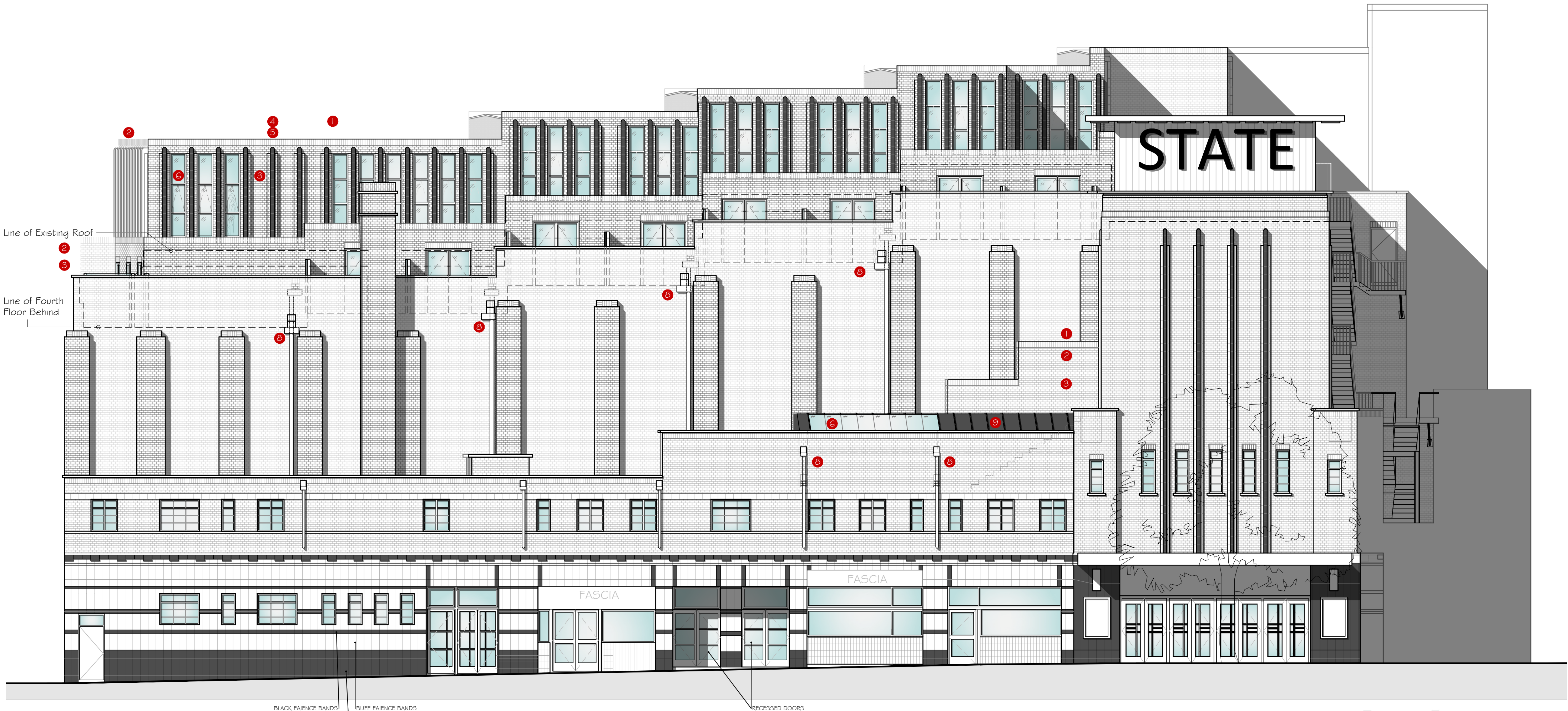
SOUTH ELEVATION
