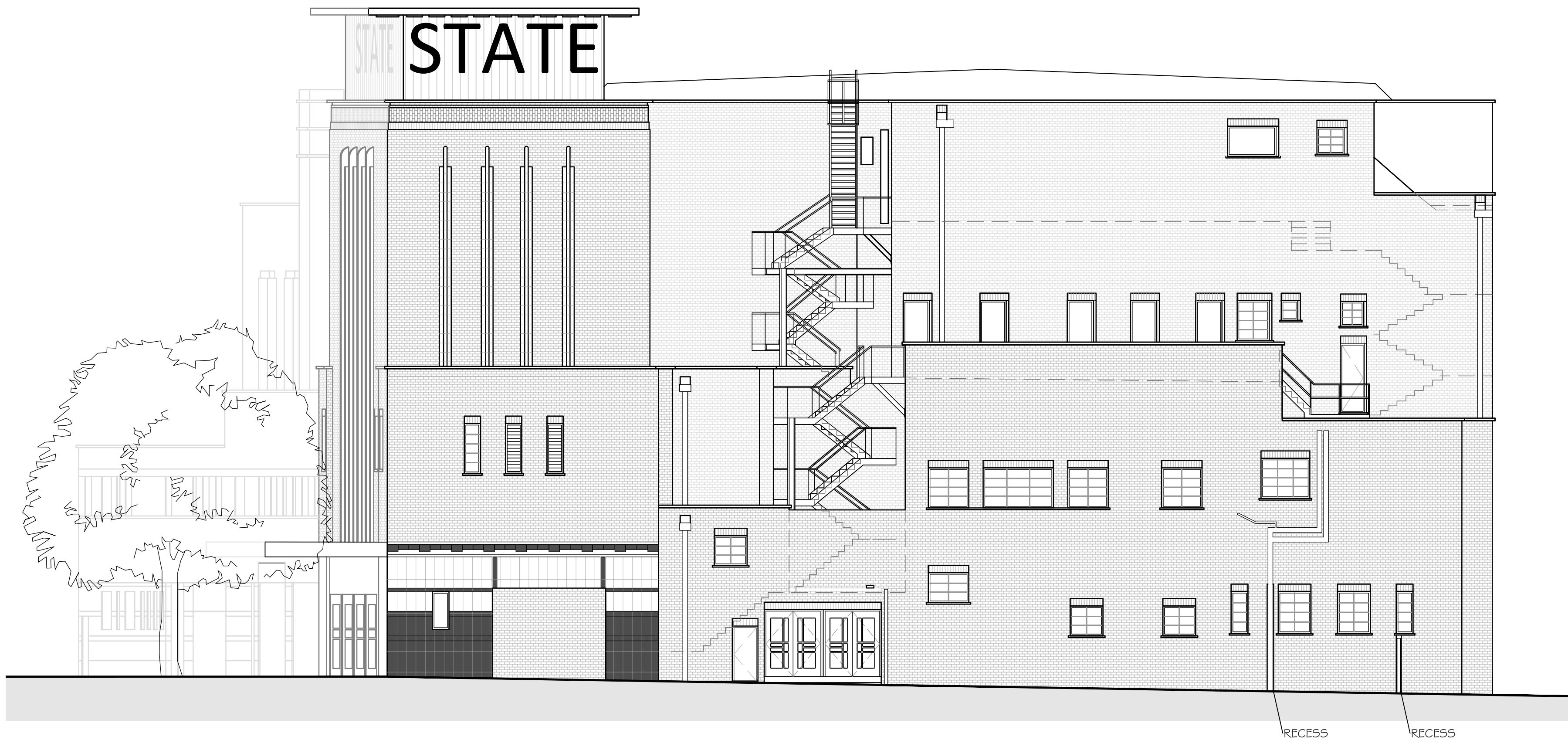
EAST ELEVATION
