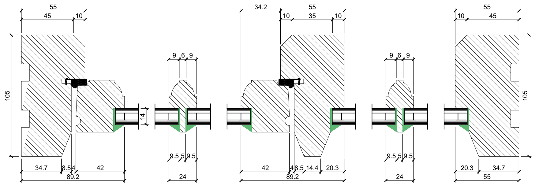
TYPICAL DETAILS OF TIMBER WINDOW, SCALE 1:10 & 1:5
